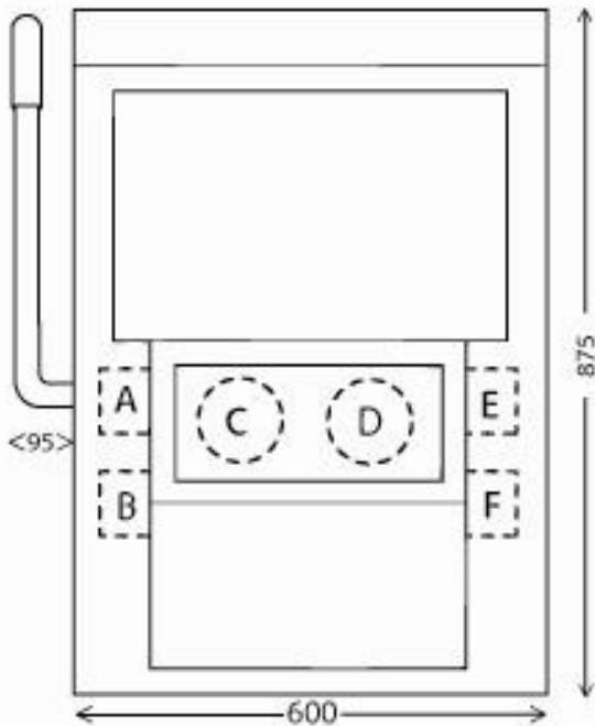
Diagram of the reverse of the unit showing all possible inlet positions for the inlet box.
